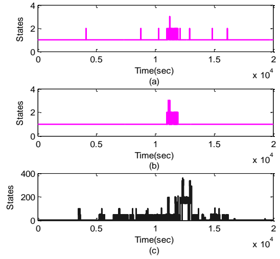
Fig 4.7. Washing-machine’s disaggregation, Disaggregated Washing-machine’s Viterbi state sequence (a) from combined Viterbi state sequence(c), and known generated washing-machine Viterbi state sequence (b)
